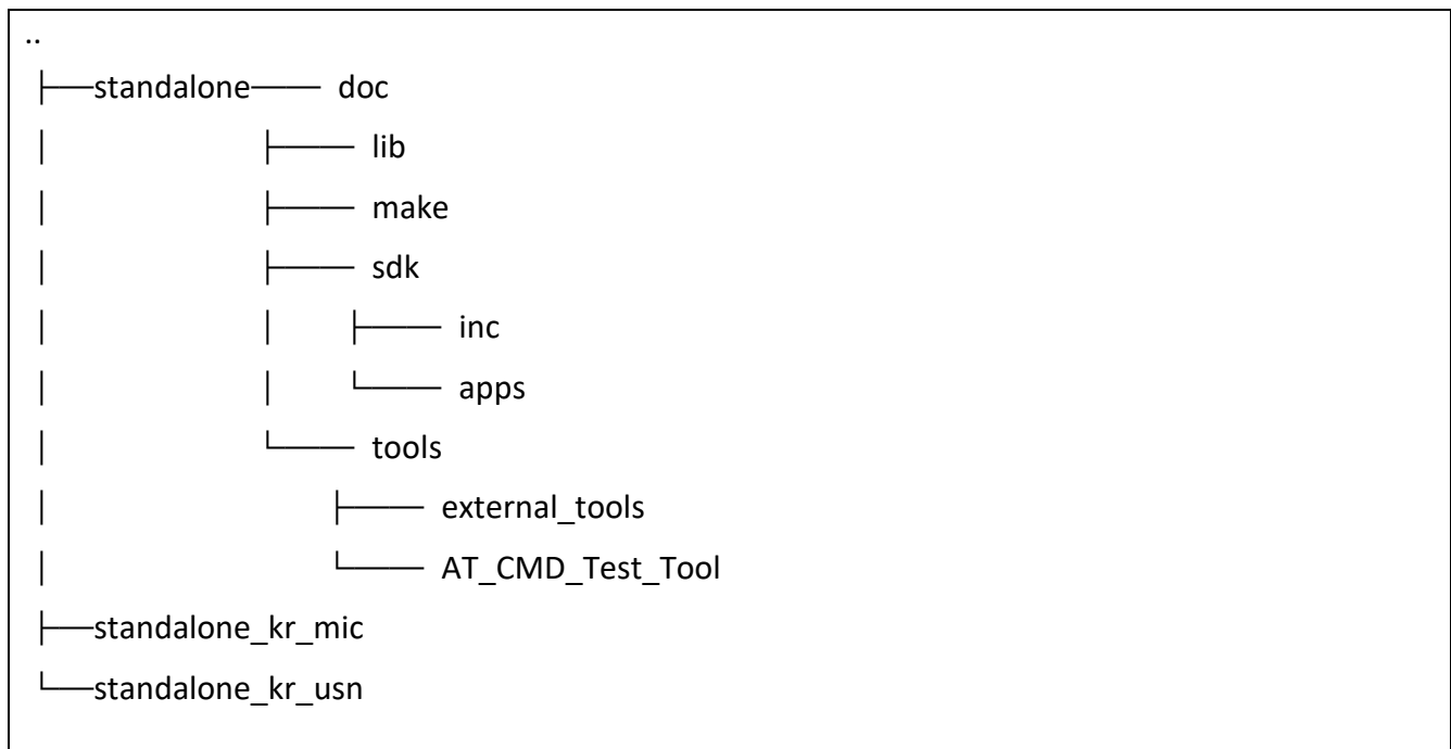
Figure 2.1 NRC7292 standalone SDK package directory
